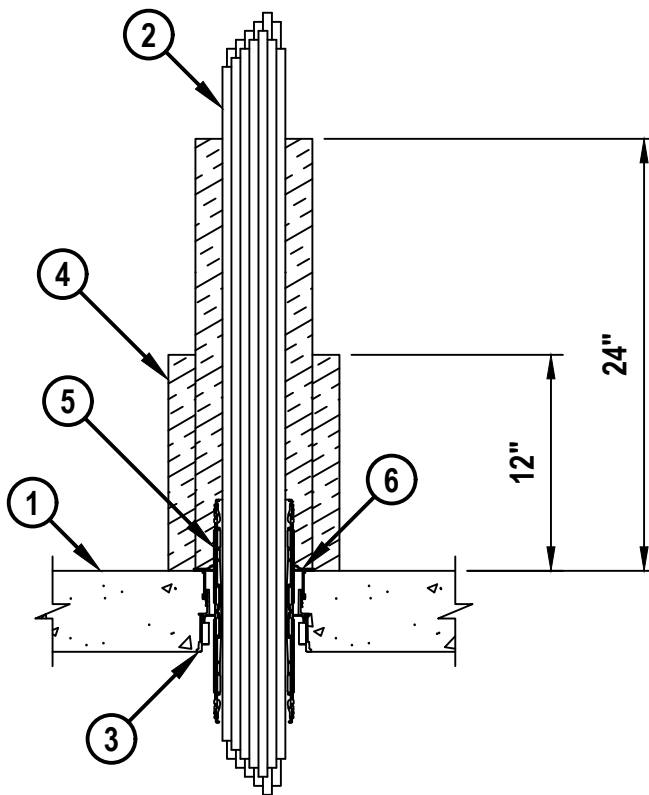
SECTION B-B
